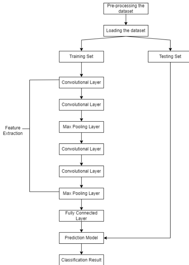
Fig. 5. Flowchart of CNN Model 1 for Devanagari Consonants and Numerals
